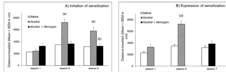
Fig 2. Effect of a treatment by ifenprodil + cyproheptadine in combination on alcohol induced sensitization. Y axis: distance travelled in cm (mean ± S.E.M.) A) Initiation of sensitization Session 1: all groups (N = 8 animals per group) received two saline administrations, 15 min and 30 min after being placed in the actimeter. Sessions 2 to 8: groups received saline or ifenprodil 1 mg/kg + cyproheptadine 1 mg/kg and then saline or alcohol (1g/kg ip/session), as indicated in materials and methods. Statistical analyses: repeated measures ANOVA, group effect F_{2;21} = 14.2, p < 0.001 , session effect F_{2;42} = 22.6, p < 0.001 , group × session interaction F_{4;42} = 9.5, p < 0.001 ; one-way ANOVAs, differences between groups in session 1 F_{2;21} = 2.2, p = ns ; in session 6 F_{2;21} = 21.7, p < 0.001 , in session 8 F_{2;21} = 8.3, p < 0.01 ; post-hoc comparisons, Bonferroni/Dunn test, (a) significantly different ( p < 0.05 ) from saline group; (b) significantly different ( p < 0.05 ) from alcohol group. B) Expression of sensitization: all animals (N = 8 animals per group) received alcohol and no further treatment until session 7. At session 7, animals sensitized to alcohol received ifenprodil (1 mg/kg) + cyproheptadine (1 mg/kg) before alcohol administration (1 g/kg, ip). Statistical analyses: repeated measures ANOVA, group effect F_{1;14} = 30.9, p < 0.001 , session effect F_{2;28} = 19.0, p < 0.001 , group × session interaction F_{2;28} = 7.6, p < 0.01 ; Student's t-test, (a) significantly different ( p < 0.05 ) from saline group.
